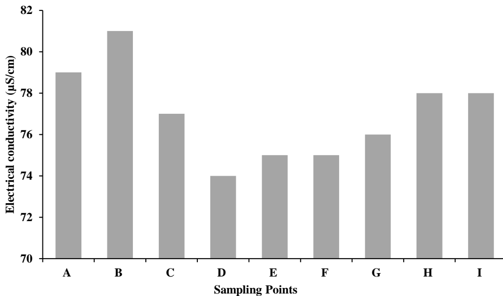
Fig. 2. Levels of electrical conductivity of water in the Bontanga irrigation dam
