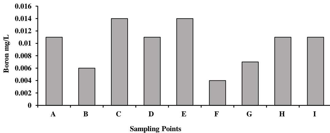
Fig. 17. Levels of Boron in the water of the Bontanga irrigation dam
