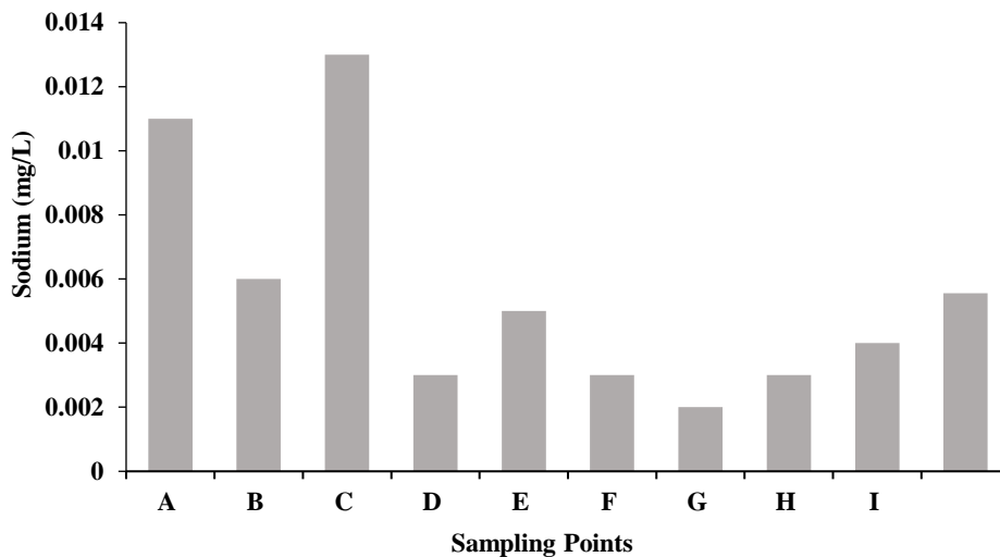
Fig. 11. Levels of sodium in the water of the Bontanga irrigation dam
