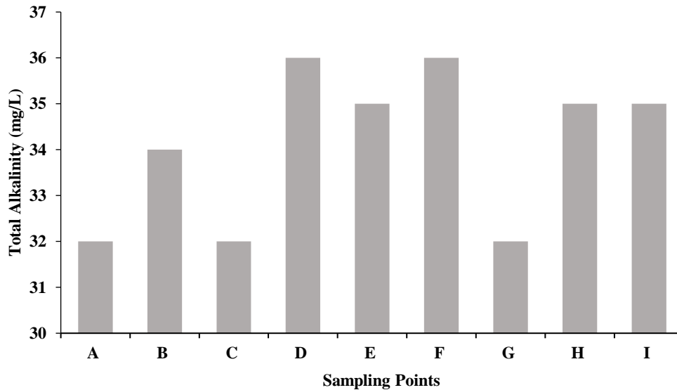
Fig. 10. Levels of total alkalinity in the water of the Bontanga irrigation dam
