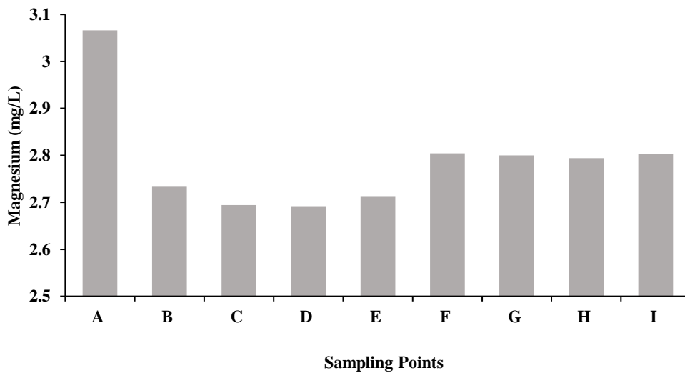
Fig. 15. Levels of magnesium in the water of the Bontanga irrigation dam
