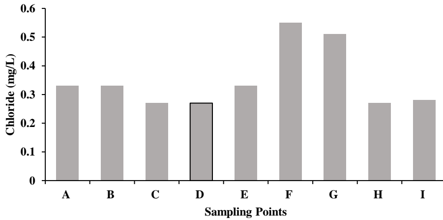
Fig. 13. Levels of chloride in the water of the Bontanga irrigation dam
