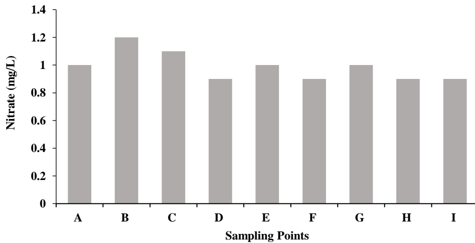
Fig. 5. Levels of nitrate ( \text{NO}_3 ) in the water of the Bontanga irrigation dam
