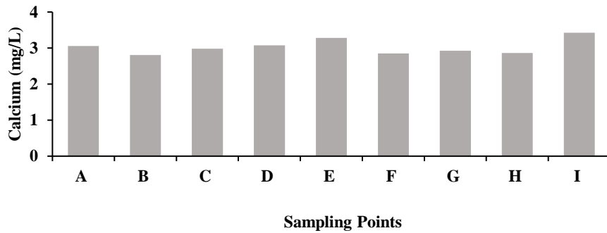
Fig. 16. Levels of calcium in the water of the Bontanga irrigation dam
