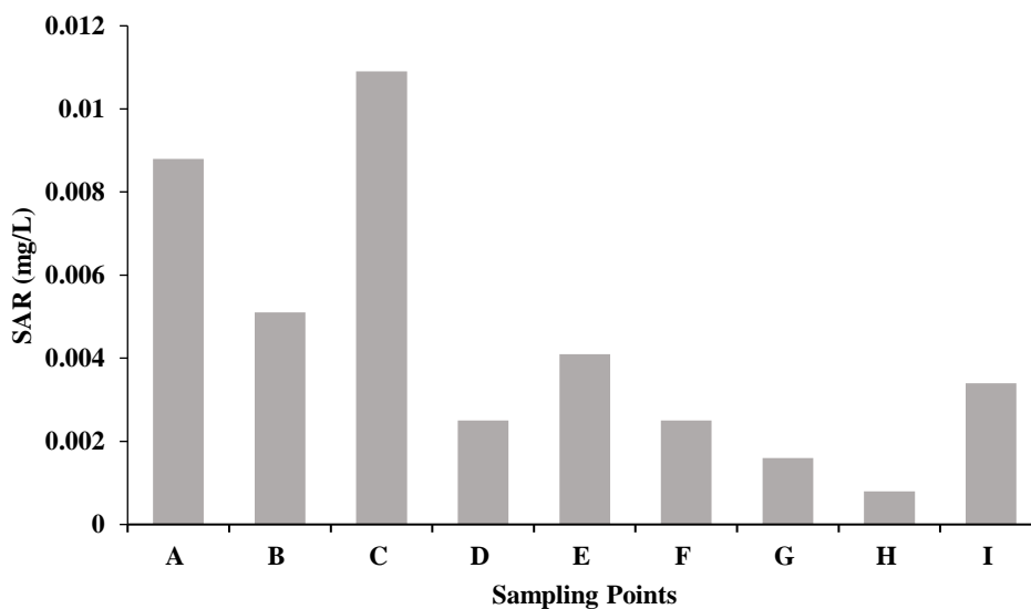
Fig. 12. Levels of SAR in the water of the Bontanga irrigation dam
