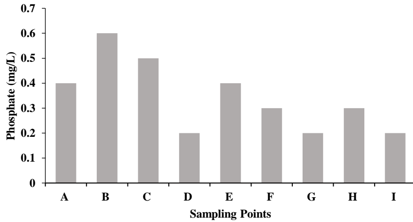
Fig. 6. Levels of PO_4 -P in the water of the Bontanga irrigation dam
