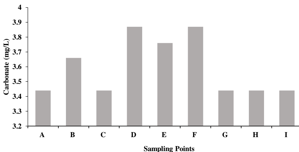
Fig. 9. Levels of carbonate in the water of the Bontanga irrigation dam
