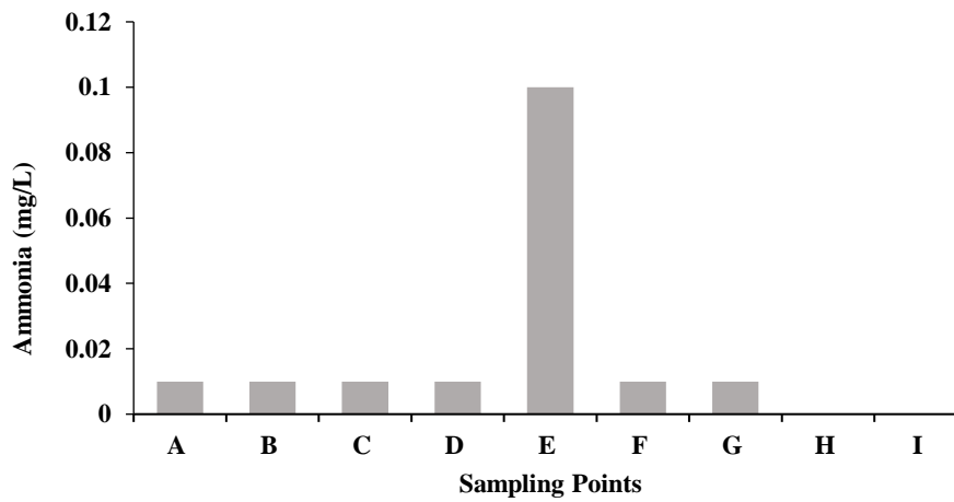
Fig. 7. Levels of Ammonia in the water of the Bontanga irrigation dam
