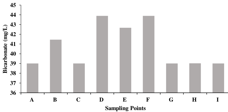
Fig. 8. Level of bicarbonate in the water of the Bontanga irrigation dam
