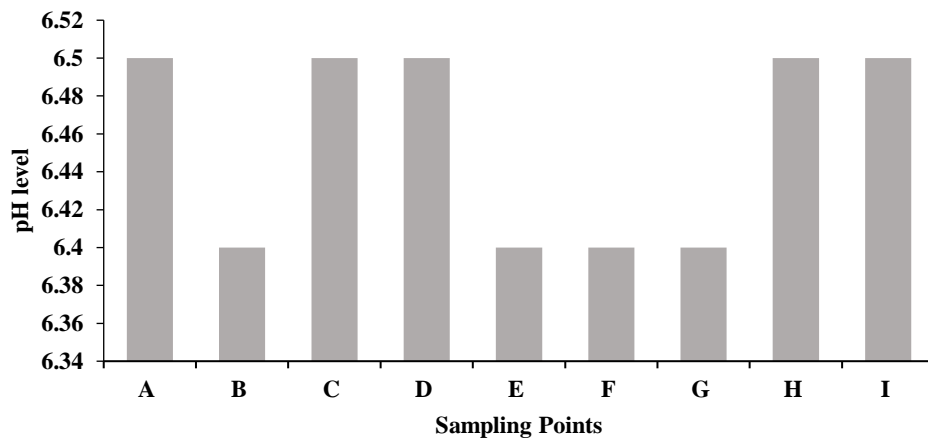
Fig. 4. Levels of pH of water in the Bontanga irrigation dam
