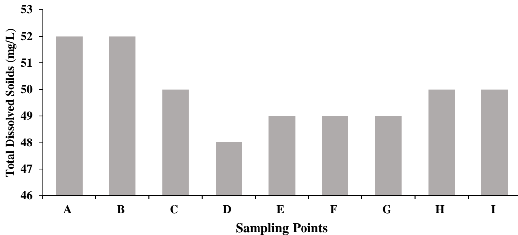
Fig. 3. Levels of total dissolved solids in the water of the Bontanga irrigation dam
