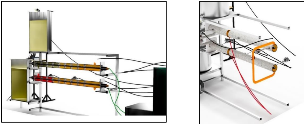
Fig. 7. Sectional parts for designed ohmic heater (Auto CAD drawings)
