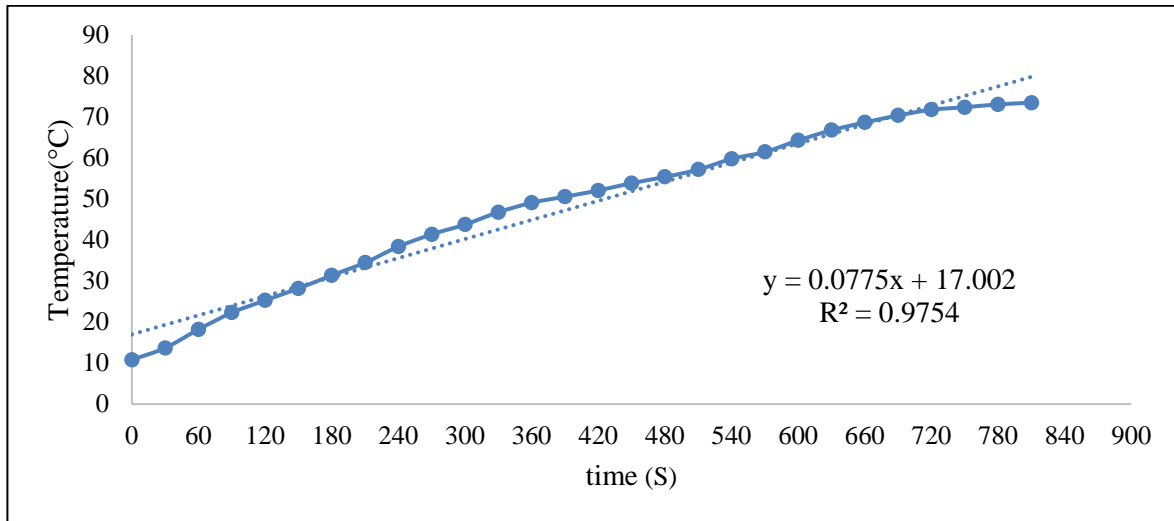
Fig. 8. Temperature profile during ohmic heating for standardized milk
