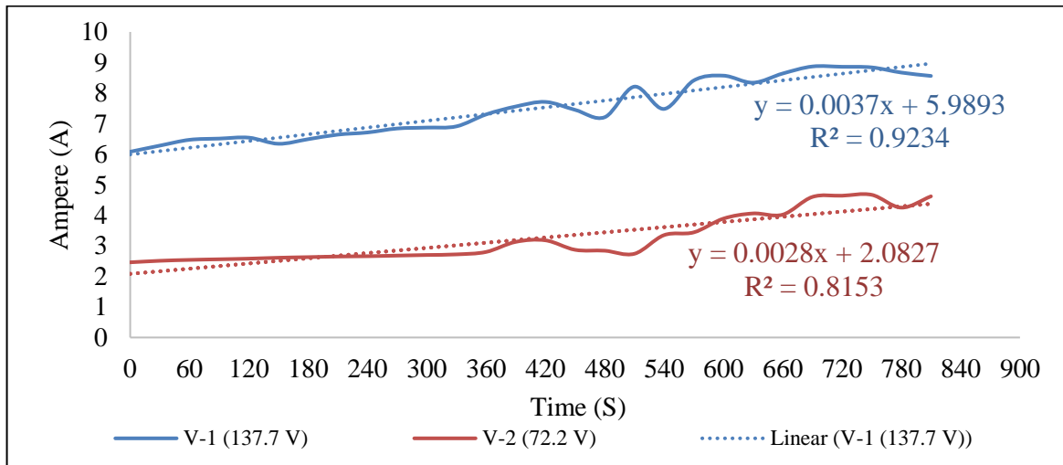
Fig. 9. Current profile during ohmic heating for standardized milk
