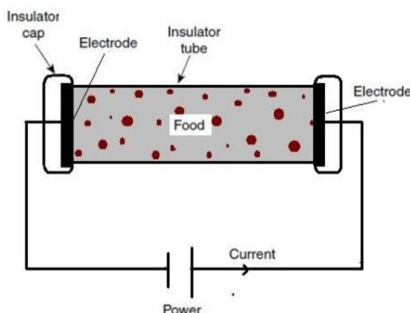
Fig. 1. Principle of ohmic heating
