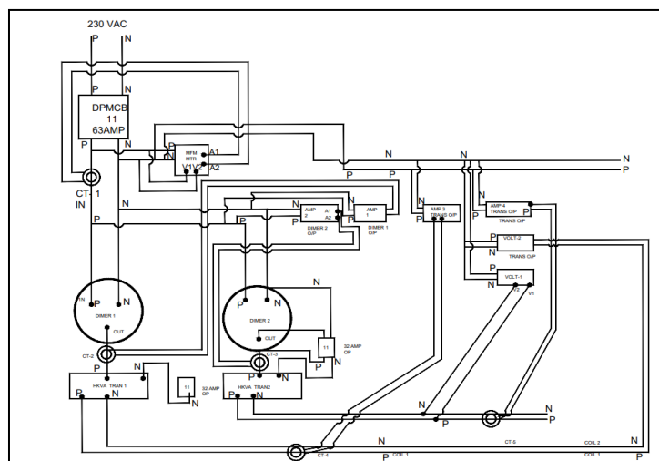
Fig. 4. Technical drawing of control panel
