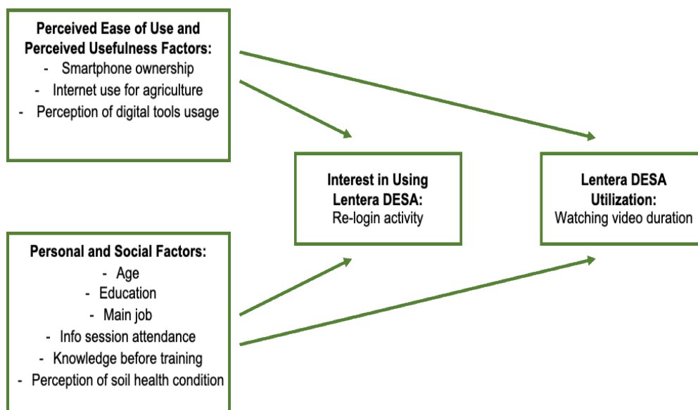
Fig. 1. Research Framework
