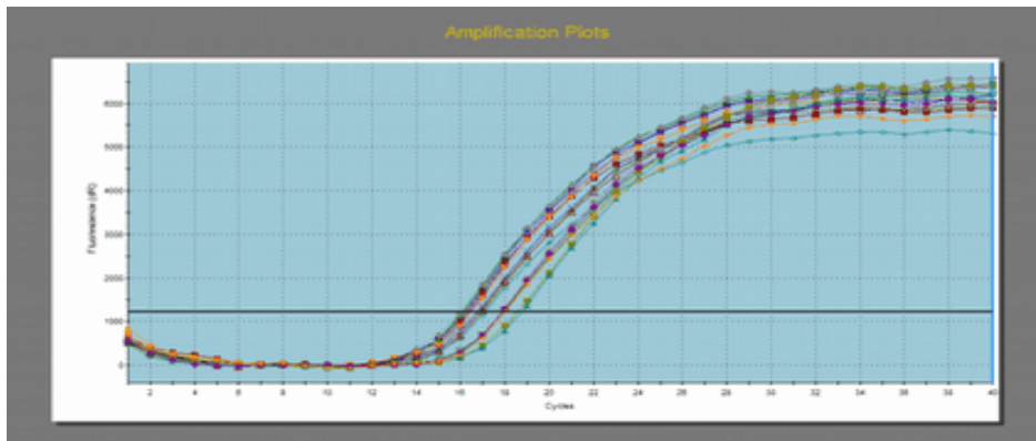
Fig. 6. Amplification Plots of SIR2 primer, 16 curves (each Ct value in given in Table 3)
