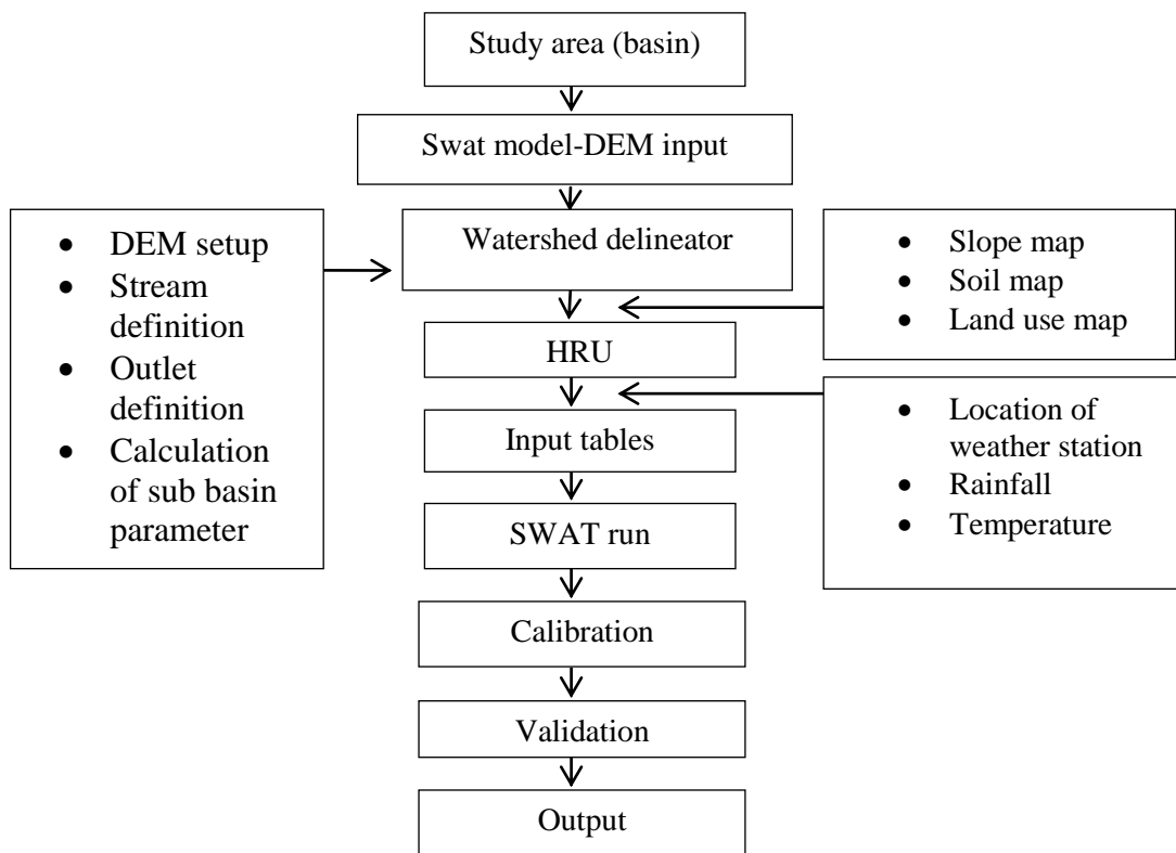
Fig. 2. Procedure followed for the SWAT modeling
