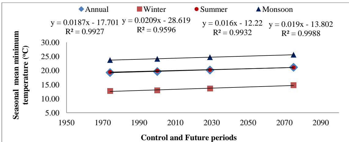
Fig. 7. Comparison of seasonal average of minimum temperature during various seasons for different periods in Sani river basin
