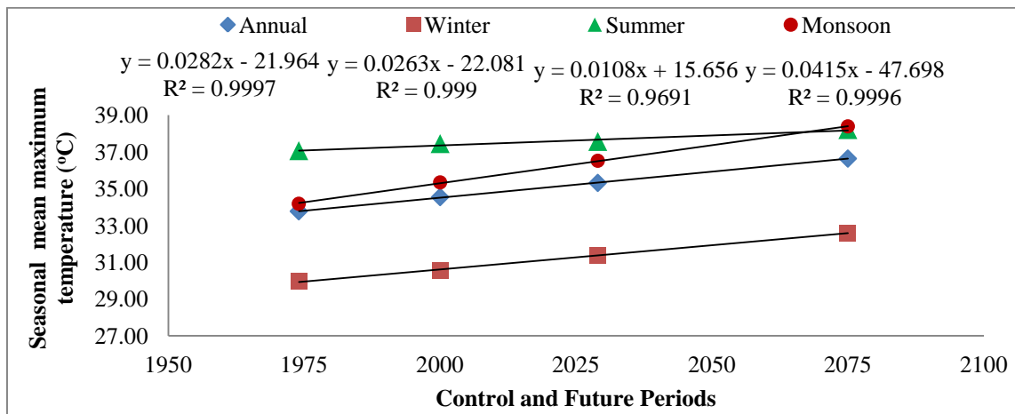
Fig. 6. Comparison of seasonal average of maximum temperature during various different seasons for different periods in Sani river basin
