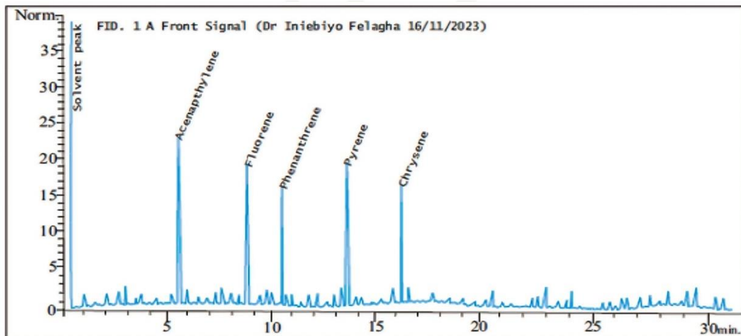
Fig. 2. GC-FID chromatogram of Ofor (Detarium microcarpum) .
