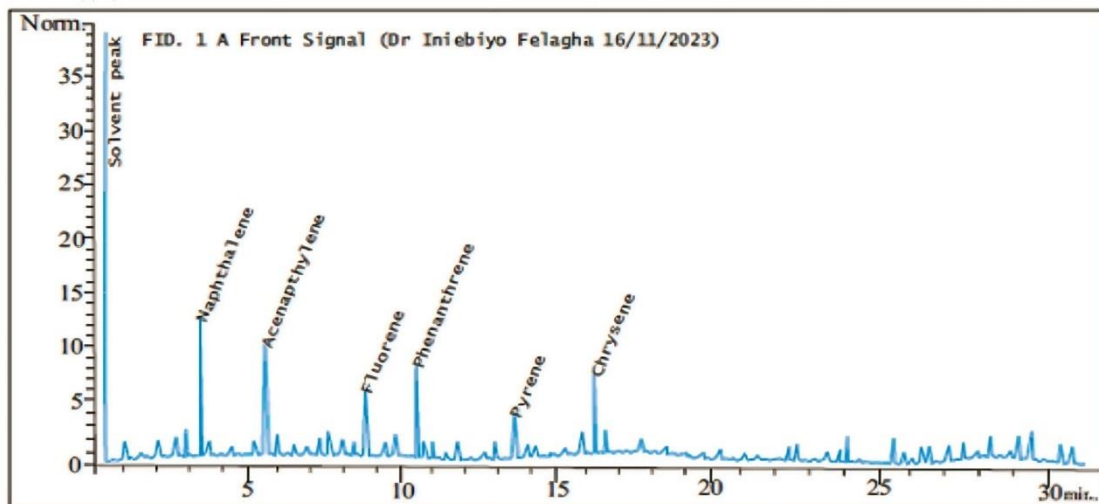
Fig. 3. GC-FID chromatogram of Ukpo (Mucuna sloanei)
